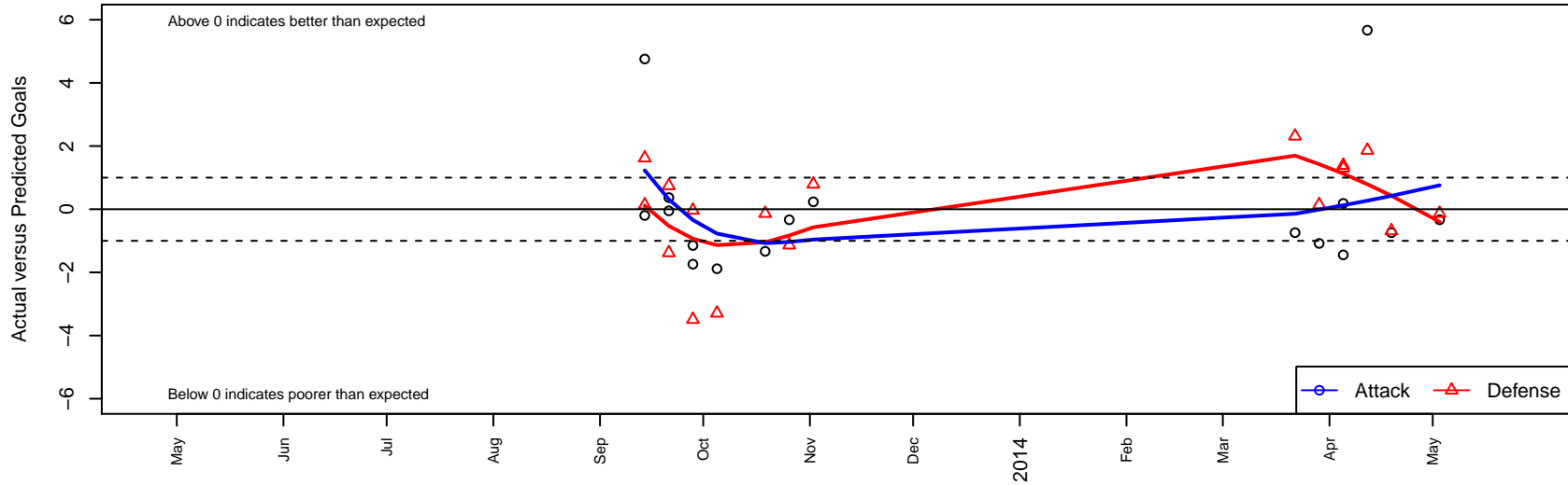
Columbia Basin YSA Dominators G02 Dots are actual minus expected GF (blue circles) and GA (red triangles). Blue line is smoothed change in attack strength. Red is smoothed change in defense strength.
